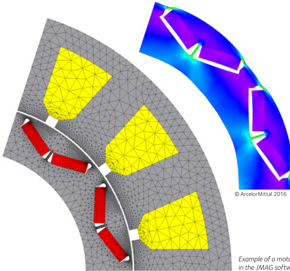
Improved mechanical stress calculations in JMAG allow designers to create smaller electrical machines
